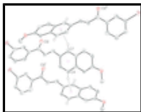
Fig. 2. Partial packing diagram for (I) showing the possible weak C—H... \pi contacts. All H atoms except H4 and H7 omitted for clarity. Symmetry codes: (i) 1/2-x, y-1/2, z ; (ii) 1-x, 1/2+y, 1/2-z .
